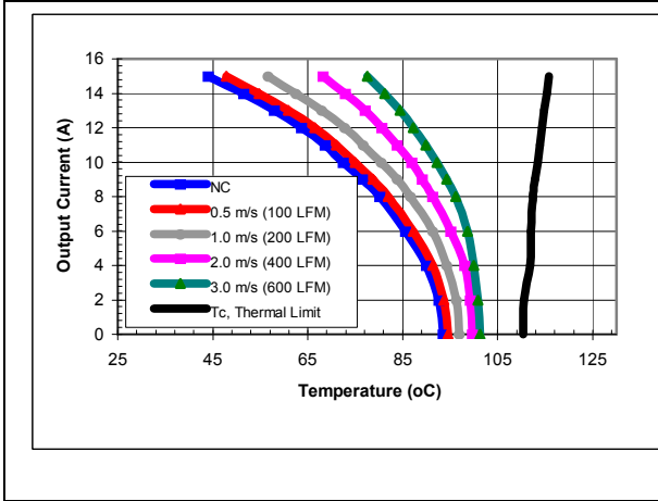
iEA48015A050V-000 maximum output current vs. ambient temperature at nominal input voltage for airflow rates natural convection (60lfm) to 600lfm with airflow from pin 3 to pin 1.
